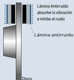
Pastilla Bosch
